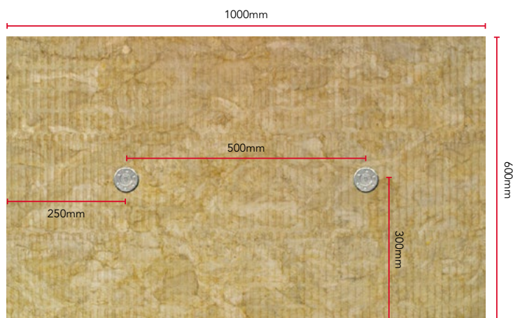
Figure 3 Inner layer fixing pattern when installing a double layered system.
